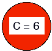
Primordial Gas Cloud
